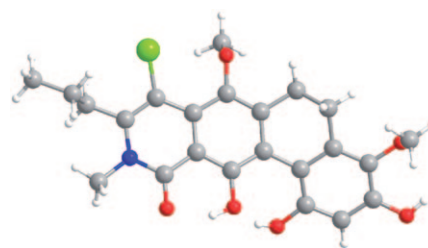
Figure 4. X-ray crystal structure of 19 . Cl green, O red, N blue, C gray, H white.
