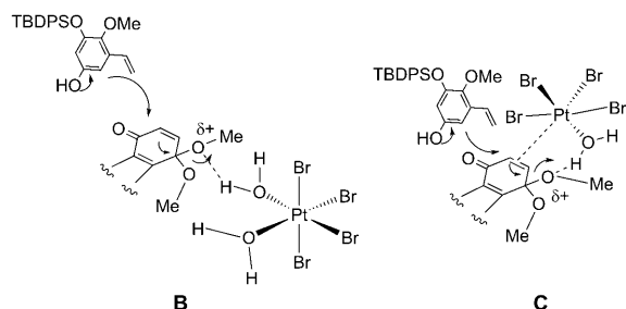
Figure 3. Possible active intermediates for Pt^{IV} -mediated arylation.
