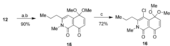
Scheme 3. Reagents and conditions: a) BCl 3 , THF, −78 °C–RT; b) PIDA, MeOH, 0 °C–RT; c) NCS, PPh 3 , DMA. PIDA = iodosobenzene diacetate, NCS = N -chlorosuccinimide, DMA = dimethylformamide.
