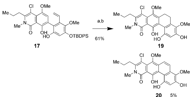
Scheme 4. Reagents and conditions: a) h\nu (Pyrex filter), cyclohexane; b) TBAF, THF 0°C. TBAF = tetrabutylammonium fluoride.
