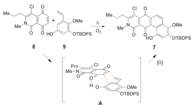
Scheme 1. Proposed cycloaddition of heterocyclic quinone 8 and styrene 9 .
