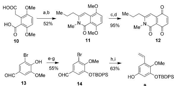
Scheme 2. Reagents and conditions: a) 2:1 pyridine:butyric anhydride reflux; b) 2.0 M MeNH 2 THF, RT, CSA, toluene, 85 °C; c) BBr 3 , THF, −78 °C–RT; d) Ag 2 O, CHCl 3 ; e) AlCl 3 , pyridine, CH 2 Cl 2 ; f) Li 2 CO 3 , MeI, DMF 45 °C; g) TBDPS-Cl, DMAP, TEA, CH 2 Cl 2 ; h) MCPBA, CH 2 Cl 2 , NaHCO 3 , MeOH 0 °C; i) vinyl tributyltin, [Pd(PPh 3 ) 4 ], toluene 85 °C; THF = tetrahydrofuran, CSA = camphor sulfonic acid, DMAP = 4-dimethylaminopyridine, MCPBA = m -chloroperoxybenzoic acid.
