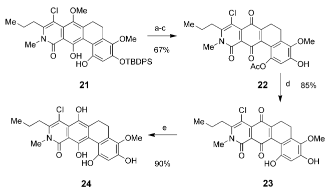
Scheme 5. Reagents and conditions: a) acetyl chloride, DIEA, \text{CH}_2\text{Cl}_2 , 0^\circ\text{C} ; b) CAN, \text{CH}_3\text{CN}/\text{pH} 7 buffer, 0^\circ\text{C} ; c) HF-pyridine, THF, 0^\circ\text{C} ; d) Otera's catalyst, 2:1 toluene:MeOH, 70^\circ\text{C} ; e) \text{Na}_2\text{S}_2\text{O}_4 , \text{H}_2\text{O}:\text{EtOAc} . DIEA = diisopropylethylamine, THF = tetrahydrofuran, CAN = ceric ammonium nitrate.
