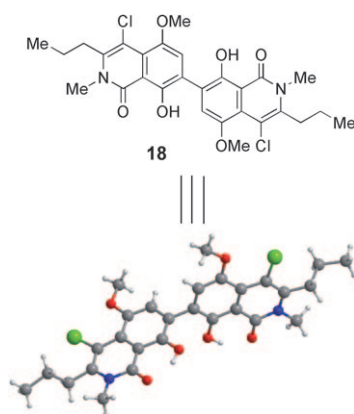
Figure 2. X-ray structure of biaryl dimer 18 . Cl green, O red, N blue, C gray, H white.
